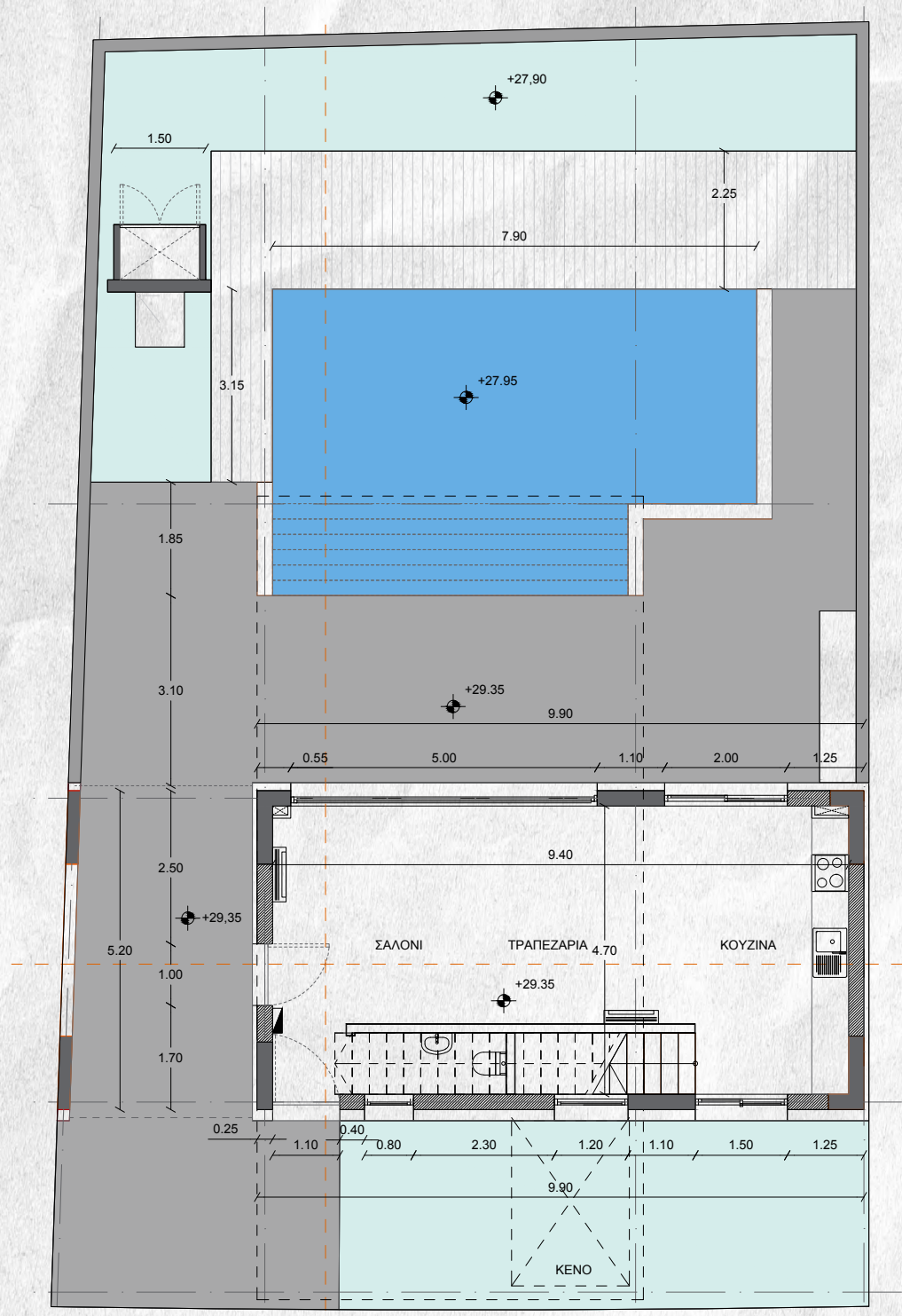
GROUND FLOOR
