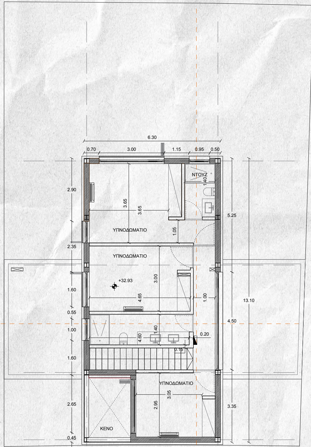
FIRST FLOOR
