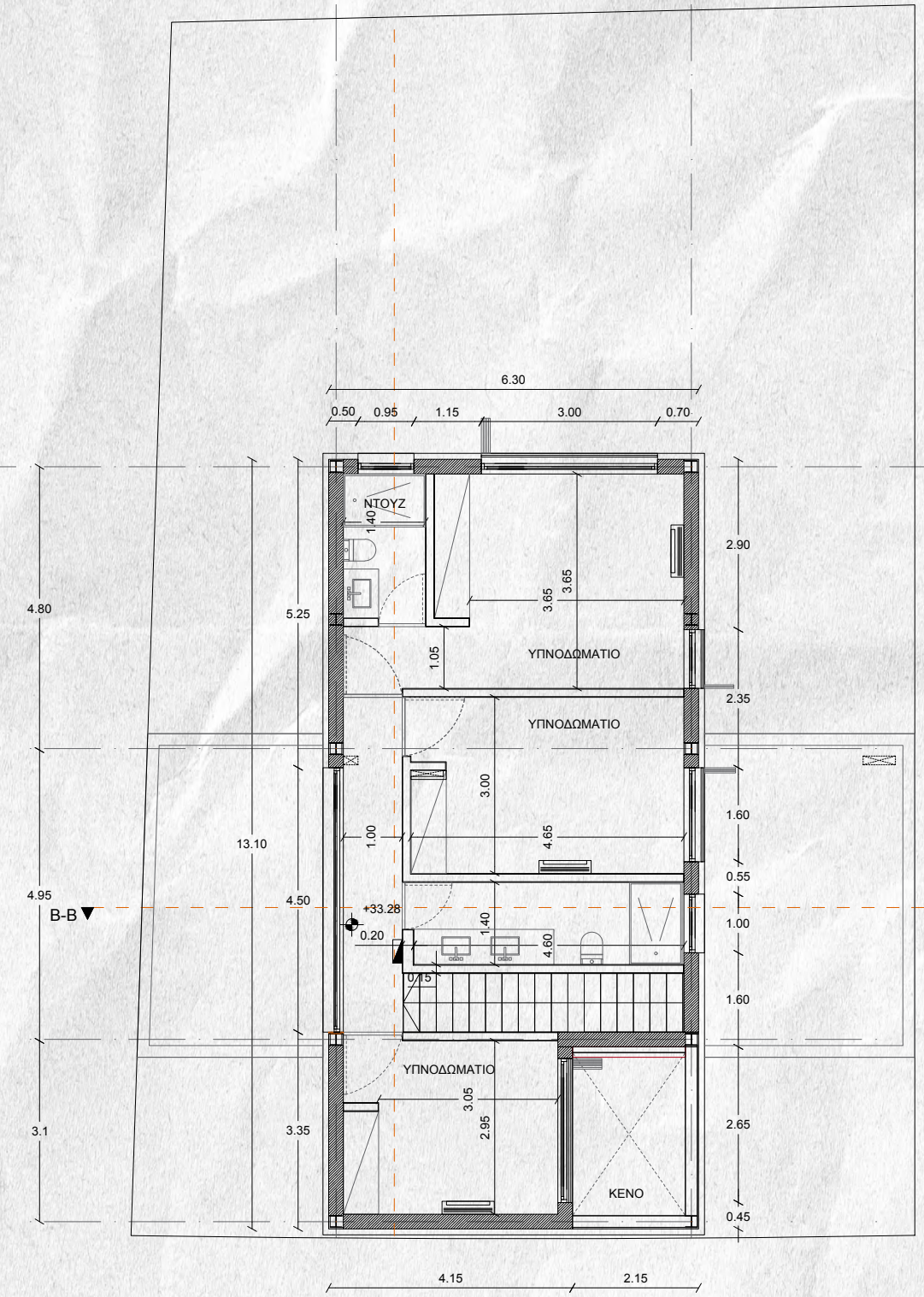
FIRST FLOOR
